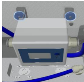
4. Unscrew each white nylon screw nut to remove from dispenser.
