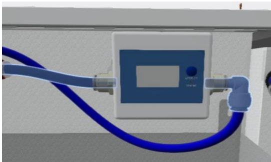
6. Re-connect poly tube and elbow to meter. Install 2-AAA batteries, and set to 2600 if new filter change is done, otherwise consult with a Wellsys service for meter setting.
